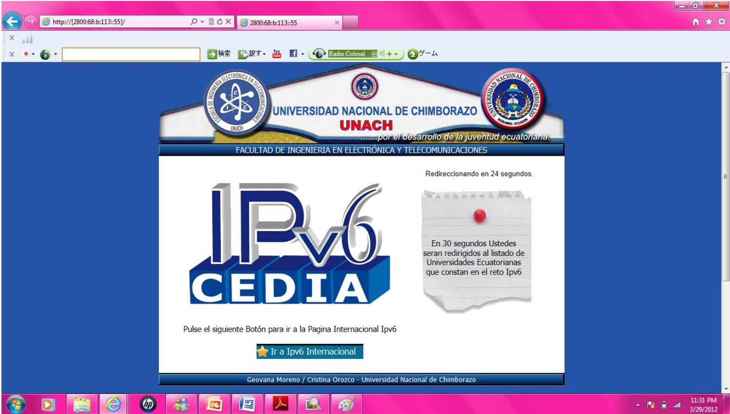
FIGURA5.5 DNS IPv6
